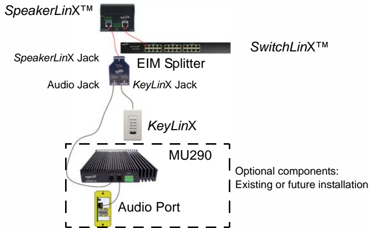
Figure 2 Connecting a KeyLinX
